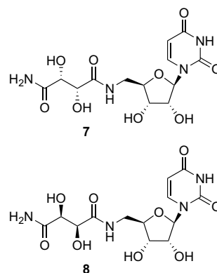
Chart 3. Uridine–tartrate UDP analogs.
