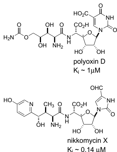
Chart 1. Naturally occurring CS inhibitors.
