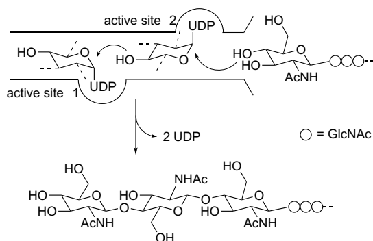
Figure 2. Proposed two site mechanism for CS.
