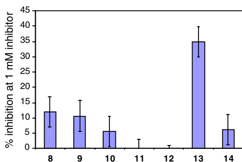
Figure 3. Inhibition of CS by 8–14 .
