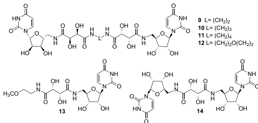
Chart 4. Uridine–tartrate dimers, linked by diamines.
