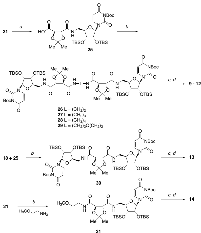
Scheme 3. Synthesis of uridine–tartrate dimers. Reagents: (a) KOH, EtOH, 99%; (b) HBTU, \text{NEt}_3 , \text{CH}_3\text{CN} , 60–80%; (c) TBAF, THF, 90%; (d) TFA, 70–80%.
