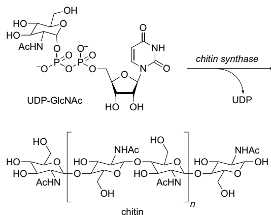
Figure 1. Biosynthesis of chitin.
