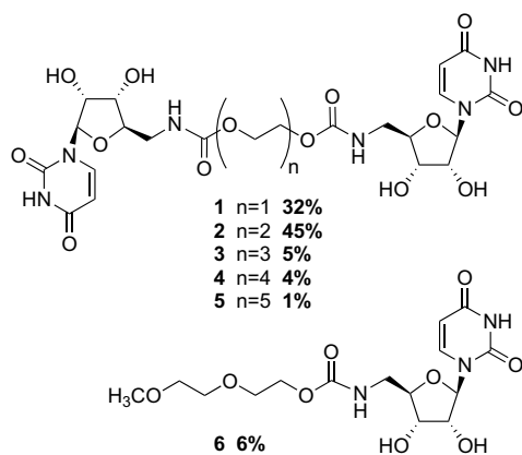
Chart 2. First-generation dimeric inhibitors, monomeric control, and inhibition of CS activity. Percentile values are % inhibition of CS activity at 1 mM inhibitor.
